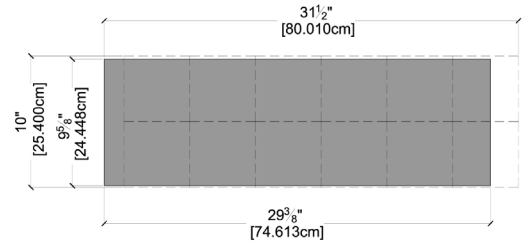
BOTTOM VIEW DIMENSIONS
